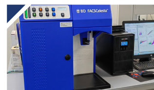
Flow Cytometry
